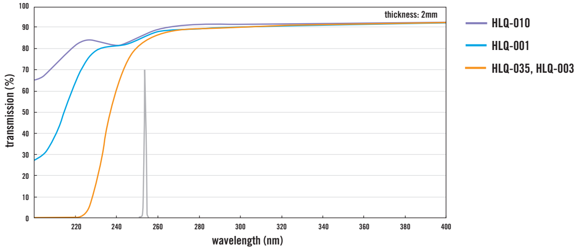
Typical transmission spectrum including reflection losses
